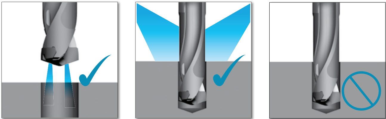
1. Internal coolant is recommended.
