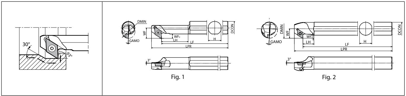
Max. Overhang Length L/D \approx 4 | Right-hand shown Right-hand Insert for Right-hand Toolholder, Left-hand Insert for Left-hand Toolholder.
