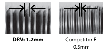
Pitch comparison of chips generated by the inner edge (Internal evaluation)
