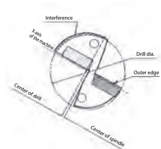
(Fig. 4) Excessive offset (For smaller hole diameter)
