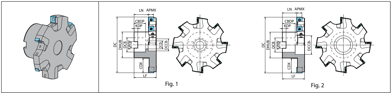
Left-hand shown
