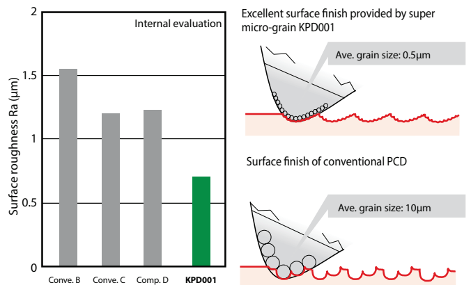
(Grain size affects surface finish quality)
