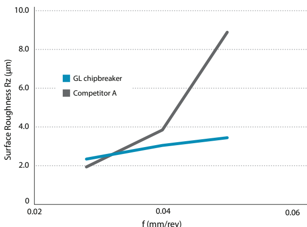
Surface roughness comparison (internal evaluation)
