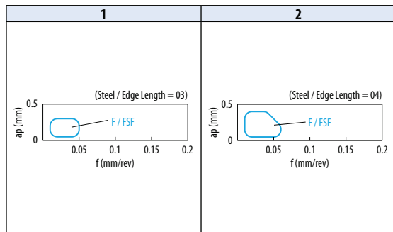
Insert whose corner-R(RE) dimension expressed with less than sign (e.g. <0.05, <0.1, <0.2 etc.) indicate models with minus tolerance on corner-R(RE).
