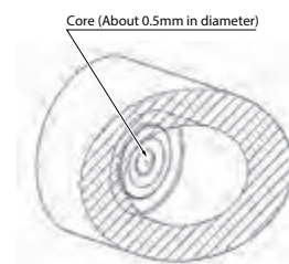
(Fig. 6) Center core
