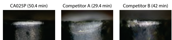
CA025P (50.4 min) Good wear condition
