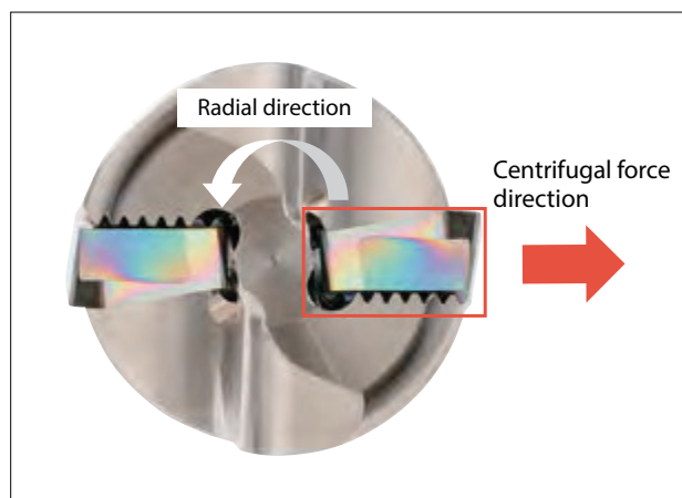
Grooved contact surface
