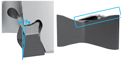
Cutting edge thickness: 5.2 mm (3.1 mm at the thinnest point) Optimized seating surface
