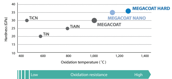
Properties of coating
