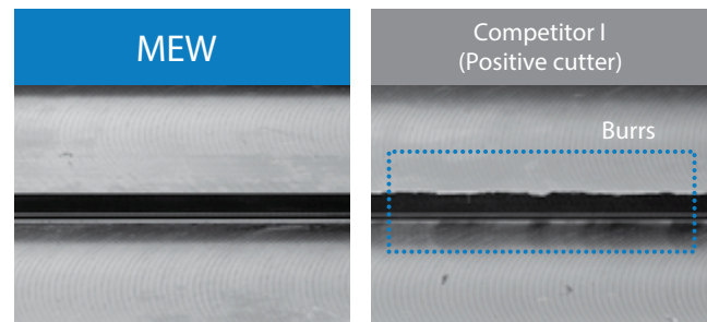
Sharp cutting enables less burrs than positive cutters
