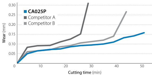
CA025P (50.4 min) Good wear condition
