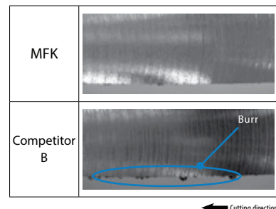
← Cutting direction
