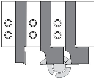
With interference
