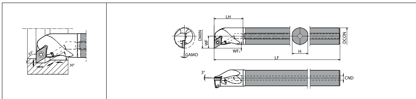
Max. Overhang Length L/D \sim 7 | Right-hand shown Left-hand Insert for Right-hand Toolholder, Right-hand Insert for Left-hand Toolholder.
