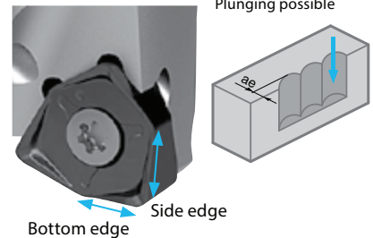
Cutting edge thickness: 5.2 mm (3.1 mm at the thinnest point) Optimized seating surface
